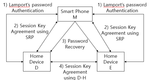
[Fig. 1] Process for session key agreement
