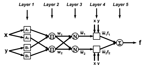
[Fig. 1] Structure of fuzzy system
