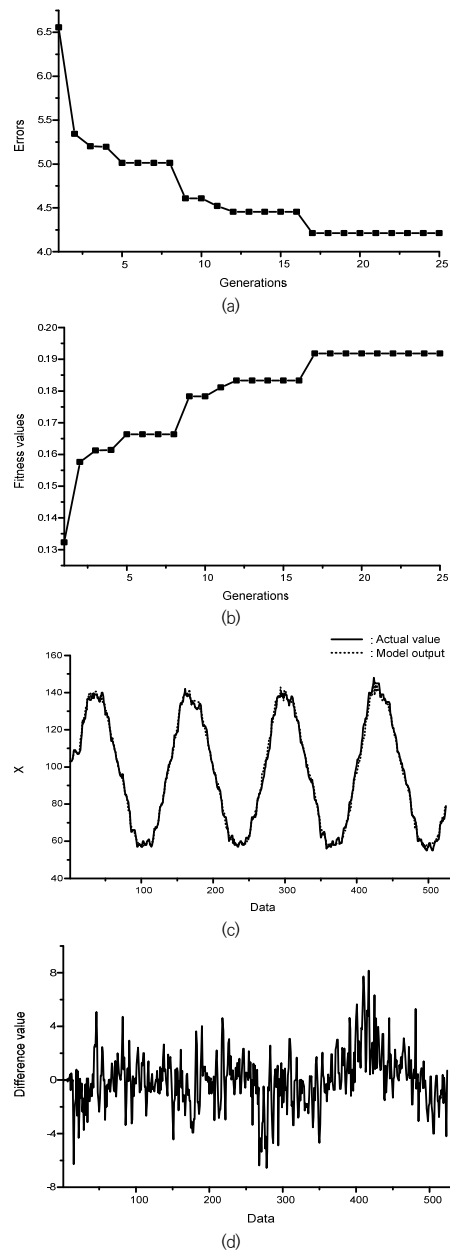
[Fig. 4] x-coordinate of the robot: (a)-MSE according to generations, (b)-fitness function values according to generations, (c)-actual values and model output, (d)-difference between actual values and model output.
