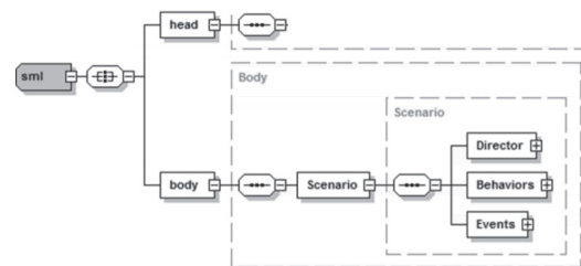
[Fig. 1] Structure of SML in [13]
