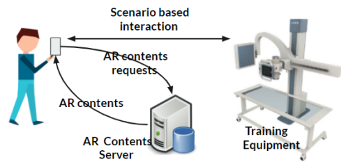
[Fig. 5] A Scenario-based AR System
