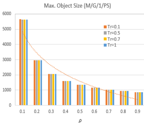
[Fig. 2] Maximum object size satisfying T_r in M/G/1/PS model
