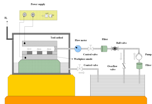
[Fig. 1] Micro-scaled flow channels ECM system
