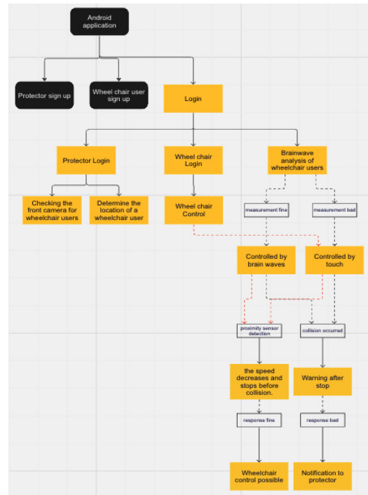
[Fig. 7] The Flow Chart of System
