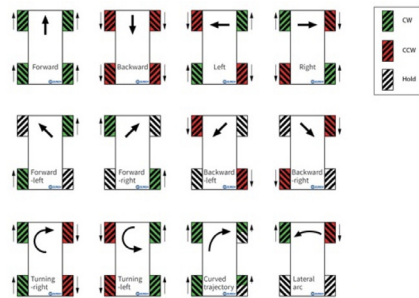
[Fig. 5] Direction of Mecanum Wheel
