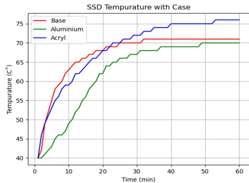
[Fig. 6] Variation by Case
