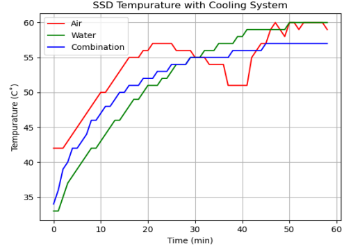
[Fig. 5] Variation by Cooling Systems
