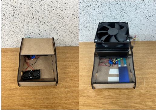
[Fig. 4] Design of Cooling System
