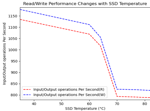
[Fig. 7] Performance Evaluation
