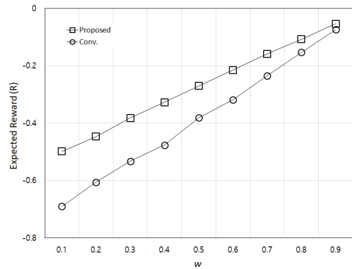
[Fig. 2] Expected reward according to \omega
