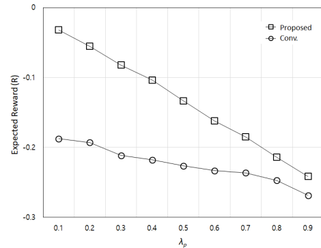
[Fig. 3] Expected reward according to \lambda_p
