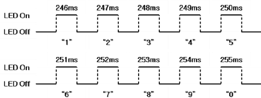
[Fig. 5] Signal scheme with blinking 250ms
