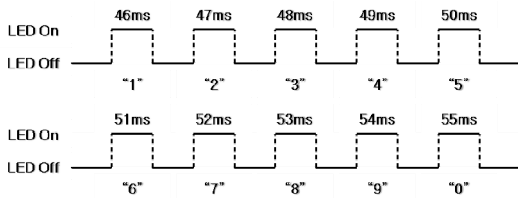
[Fig. 4] Signal scheme with blinking 50ms
