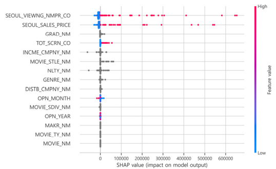
[Fig. 5] SHAP summary plot for key predictors of number of viewers in CatBoost model
