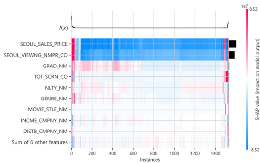
[Fig. 9] SHAP heatmap for key predictors of box office revenue in CatBoost model
