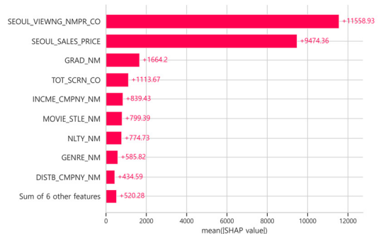
[Fig. 4] SHAP bar plot for key predictors of number of viewers in CatBoost model
