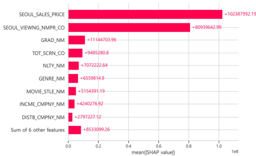
[Fig. 6] SHAP bar plot for key predictors of box office revenue in CatBoost model
