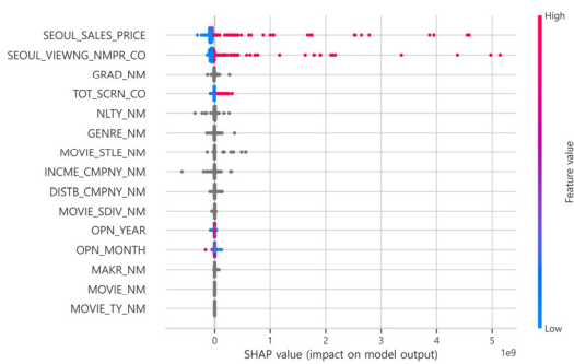
[Fig. 7] SHAP summary plot for key predictors of box office revenue in CatBoost model
