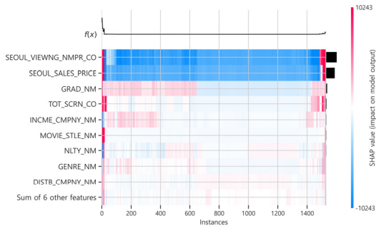
[Fig. 8] SHAP heatmap for key predictors of number of viewers in CatBoost model
