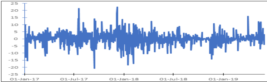
(a) Bitcoin
