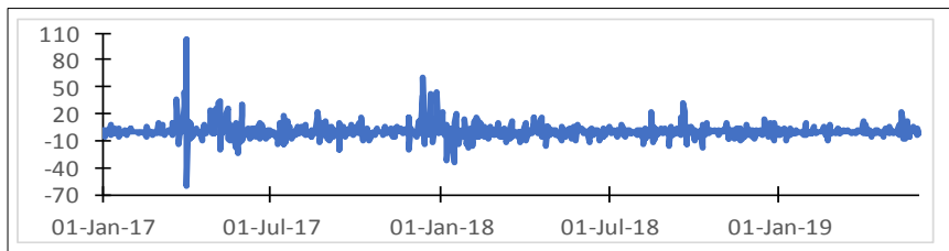
(c) Ripple
