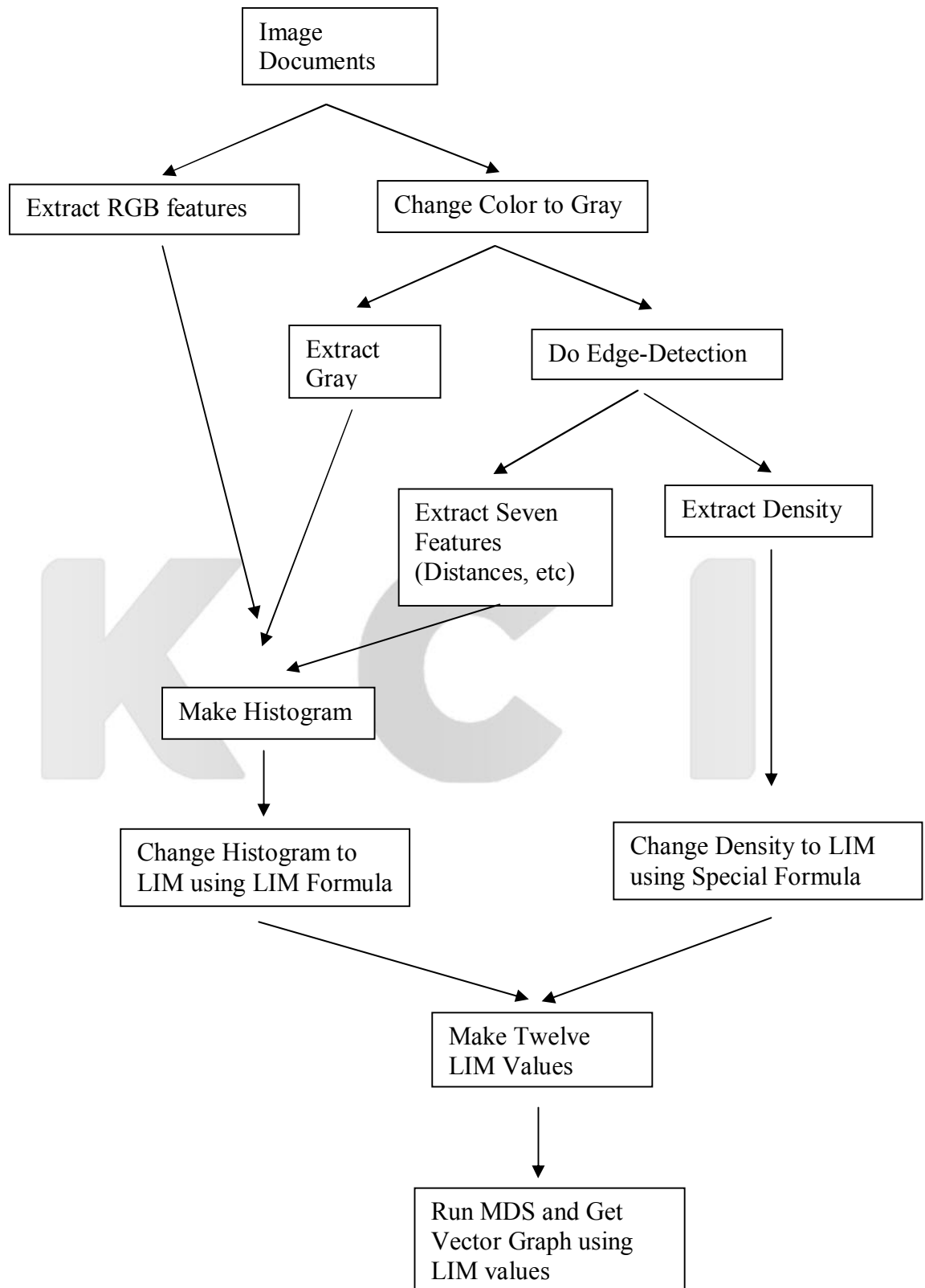
Figure 4. Flowchart for Image Document Process
