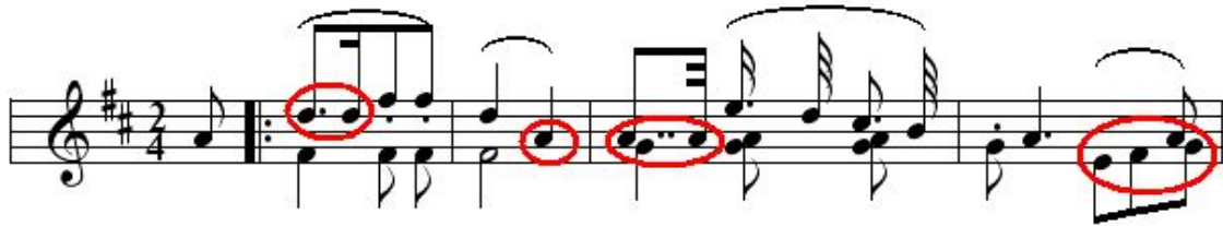
<Figure 6> Trout-Quintets
