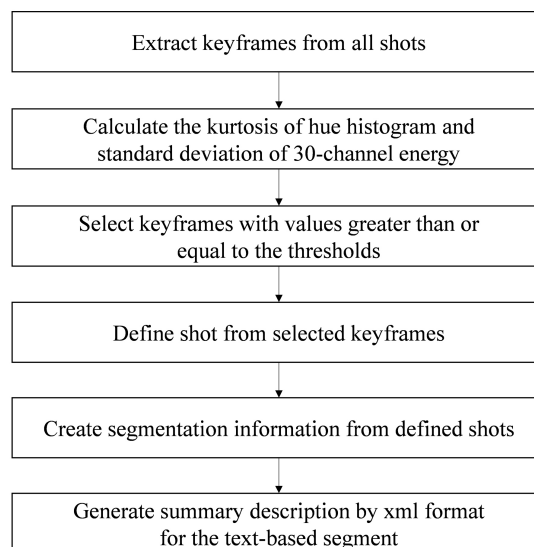
<Figure 3> Flow Chart of Detecting the Text-Based Segment
