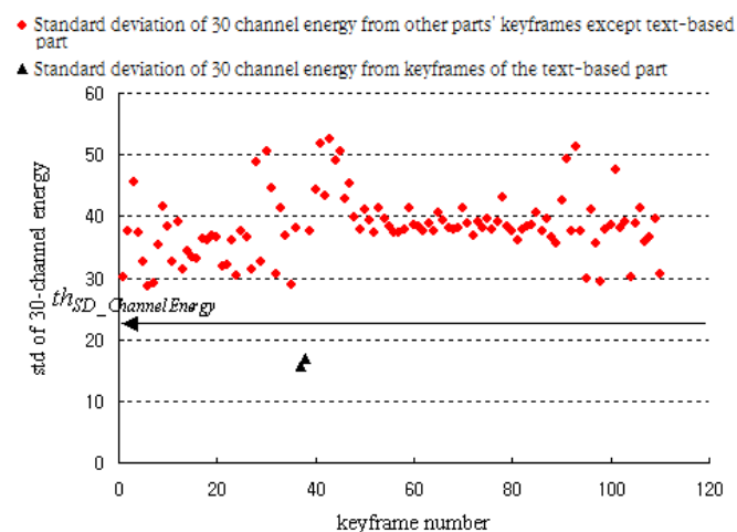
<Figure 7> 30-channel Energy Standard Deviation of Homogeneous Texture Descriptor
