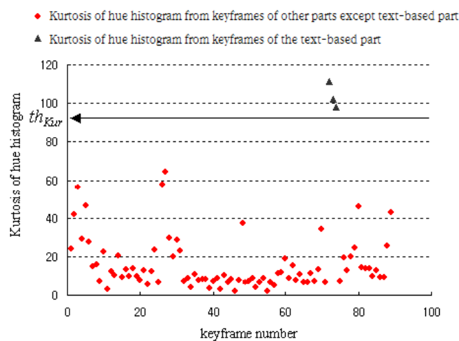
<Figure 5> Kurtosis of Hue Histogram from Keyframes
