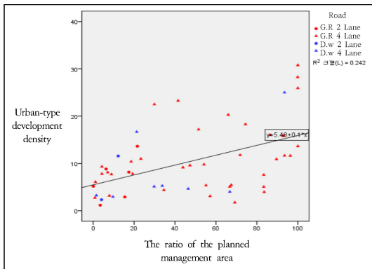
Figure 7_ Correlation Analysis between the Ratio of the Planned Management Area and the Urban-type Development Density
