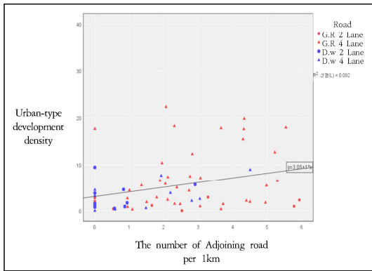
Figure 5_ Correlation Analysis between the Number of Adjoining Road per 1km and the Urban-type Development Density
