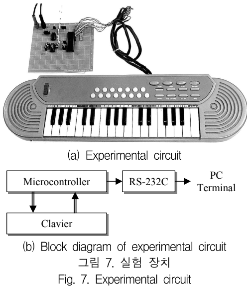
Fig. 7. Experimental circuit
