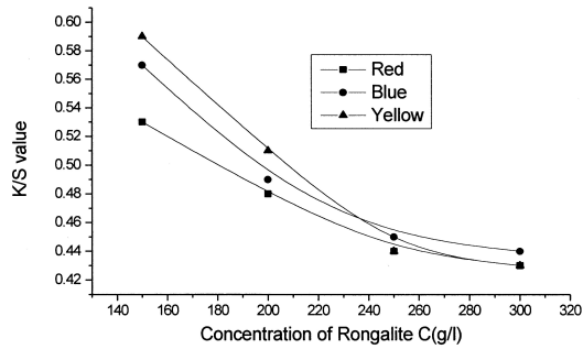
Fig. 2. Effect of concentrations of Rongalite C on K/S values of cotton fabrics dyed with Discharge Reactive dyes.
