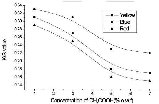
Fig. 6. Effect of concentrations of acetic acid on decoloration of cotton fabrics dyed with Discharge Reactive dyes.
