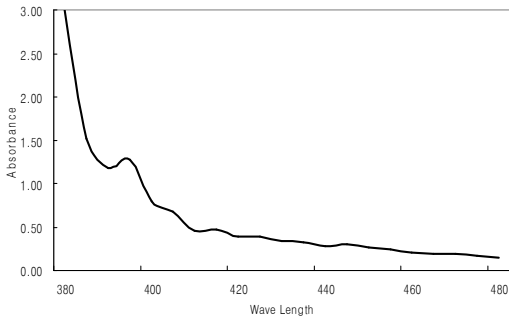
Fig. 1. Spectrum of Forsythia Koreana NAKAI (380nm-480nm)
