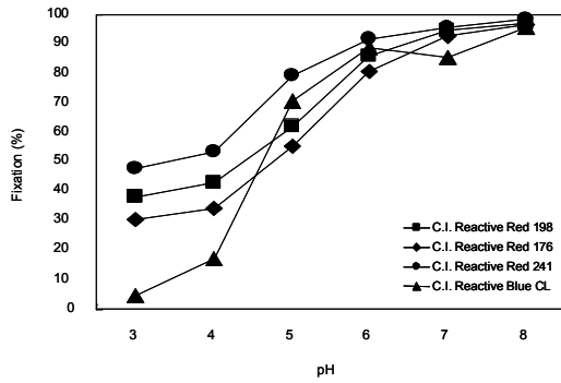
Fig. 2. Effect of application pH on fixation(%).
