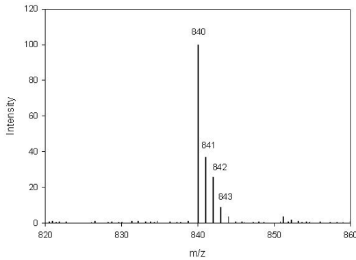
Fig. 6. Mass analysis of C. I. Reactive Red 198 at pH 12(RT 2.27min).
