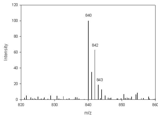
Fig. 5. Mass analysis of C. I. Reactive Red 198 at pH 5.5(RT 2.66min).
