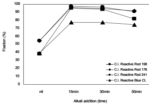
Fig. 10. Effect of alkali addition on fixation(%).
