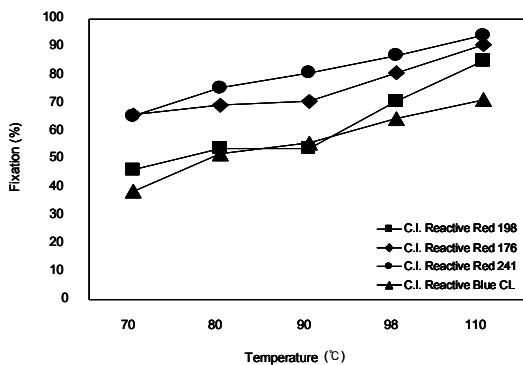
Fig. 9. Effect of application temperature on fixation(%).
