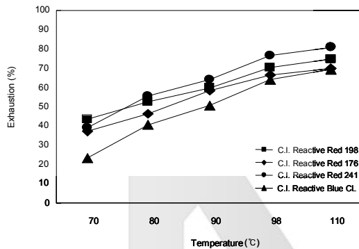
Fig. 8. Effect of application temperature on exhaustion(%).
