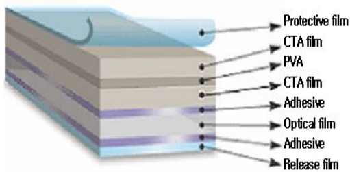
Fig. 1. Composition of polarizing film.
