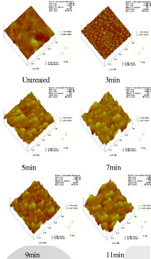
Fig. 5. AFM images on the CTA film treated with Ar low temperature plasma(at 150W).
