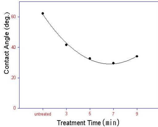
Fig. 7. Contact angle of CTA film with output power of 100W.
