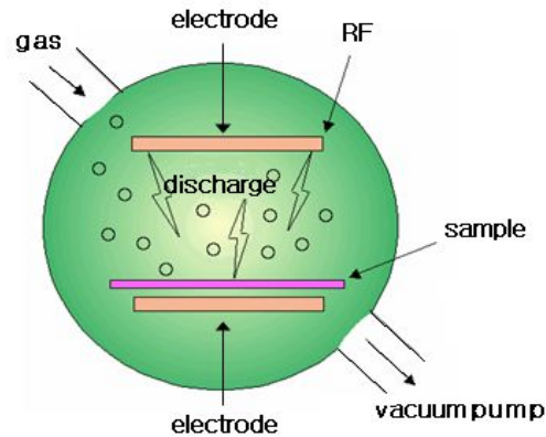
Fig. 2. Schematic diagram of low temperature plasma apparatus.
