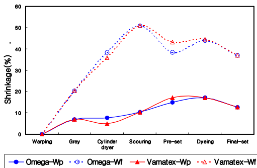
Fig. 4. Shrinkage of the fabrics according to the weaving machine.
