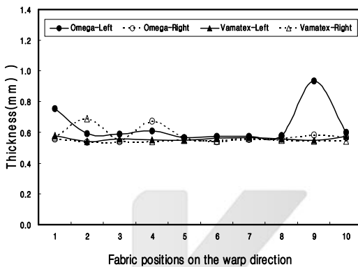
Fig. 9. The thickness variation on the right and left directions of the finished fabrics on the positions of the fabric warp direction.
