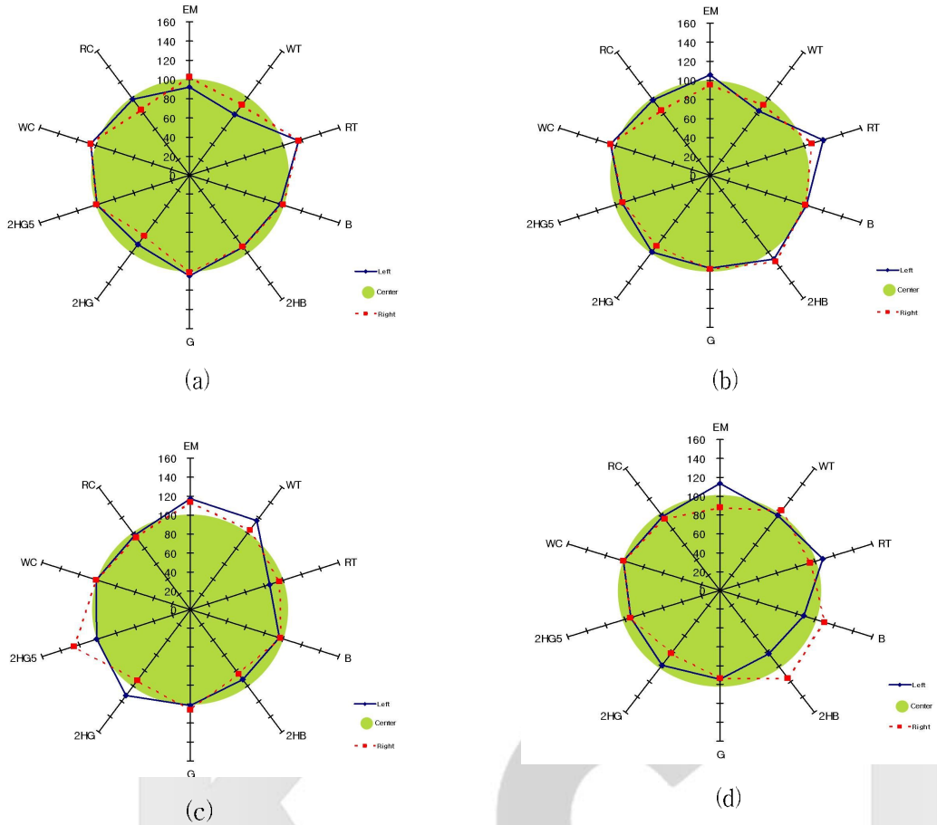
Fig.6. Thediagram of relative fabric mechanical properties between Vamatex and Omega according to the fabric positions.
