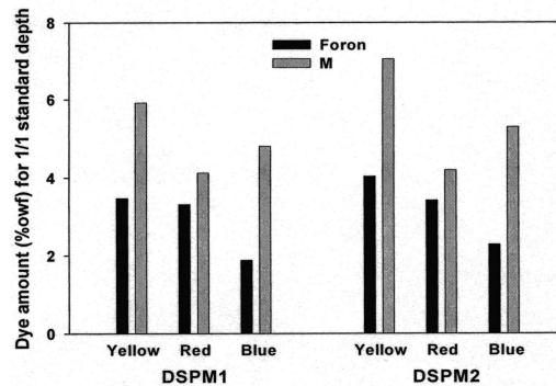
Fig. 7. Dye amount for 1/1 standard depth dyeing of direct spun type PET microfibers with disperse dyes.
