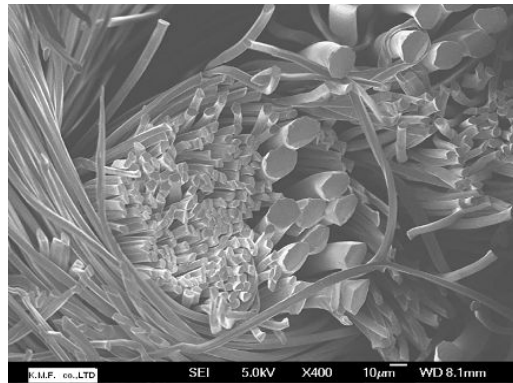
(b) DSPM2 : PET 70d/300f + High shrinkage PET 30d/12f
