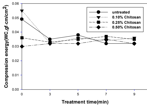
Fig. 7. Relationship between WC and plasma treatment time.
