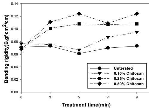
Fig. 4. Relationship between B and plasma treatment time.
