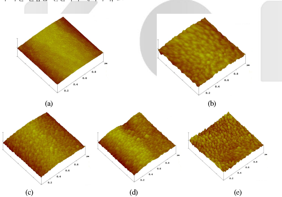
Fig. 10. AFM photographs of PET treated by plasma (a) control; (b) plasma treated for 3min; (c) plasma treated for 5min; (d) plasma treated for 7min; (e) plasma treated for 9min.
