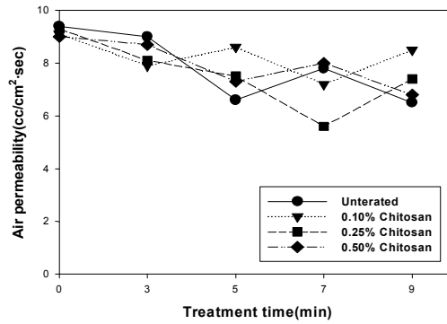
Fig. 8. Relationship between air permeability of PET treated by various chitosan concentrations and plasma treatment time.
