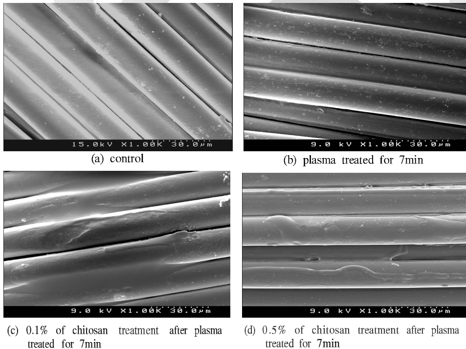
Fig. 9. SEM photographs of the PET treated with different chitosan concentration after O 2 plasma treatment.
