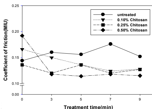
Fig. 6. Relationship between MIU and plasma treatment time.
