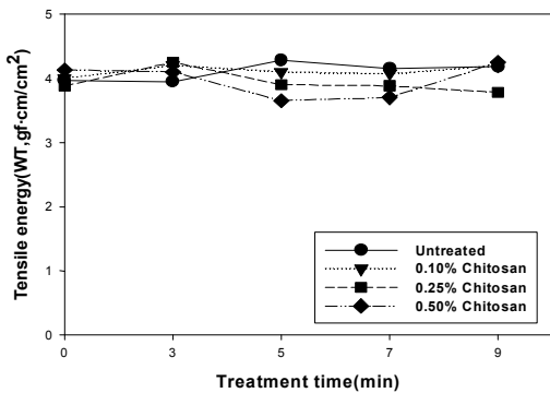
Fig. 3. Relationship between WT and plasma treatment time.
