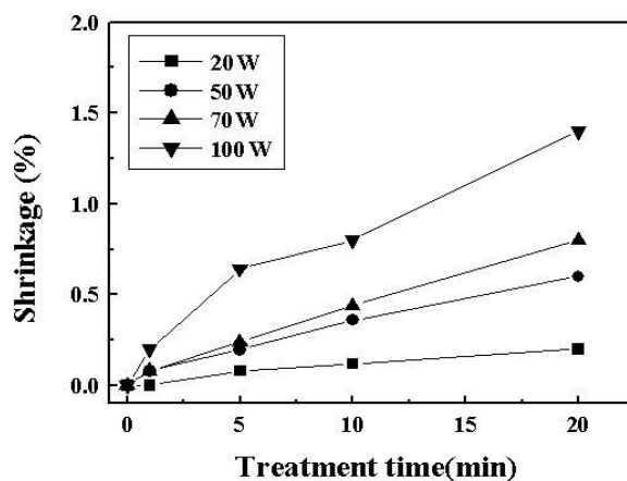
Fig. 4. Effect of plasma treatment on shrinkage of PPMB nonwovens.
