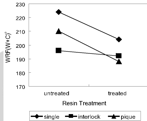
Fig. 8. Effect of laundering on wrinkle recovery angles of knitted fabrics.
