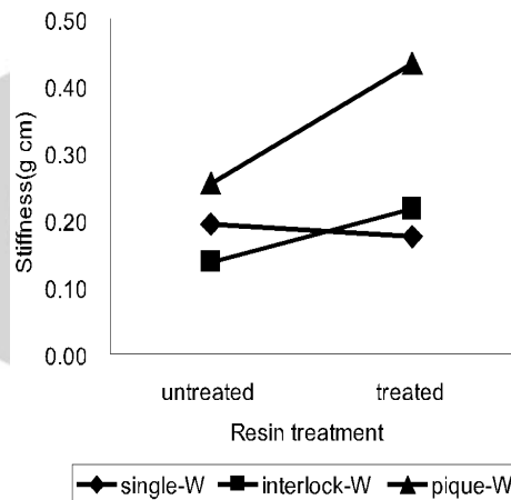
Fig. 1. Effect of resin finishing on stiffness of knitted fabrics(wale direction).
