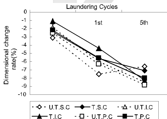
Fig. 9. Effect of laundering on dimensional stability of knitted fabrics(wale direction).
