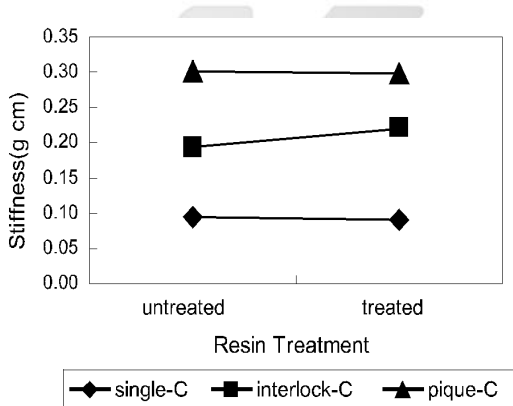
Fig. 7. Effect of laundering on stiffness of knitted fabrics(course direction).
