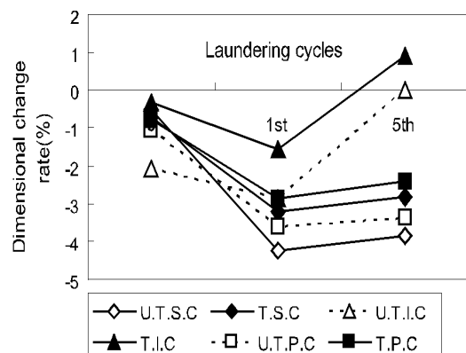
Fig. 10. Effect of laundering on dimensional stability of knitted fabrics(course direction).
