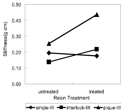
Fig. 2. Effect of resin finishing on stiffness of knitted fabrics(course direction).
