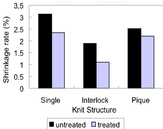
Fig. 4. Effect of resin finishing on shrinkage rate of knitted fabrics(wale direction).
