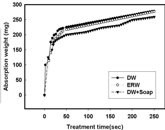
Fig. 4. Water-absorbance weight according to the treatment time on cotton fabrics.
