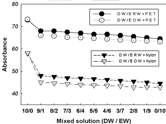
Fig. 3. Contact angle of mixed solution according to the mixing ratio on PET and Nylon films.
