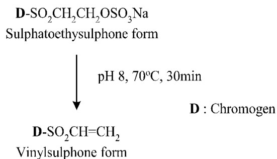
Fig. 11. Conversion of sulphatoethylsulphone form to vinylsulphone form.
