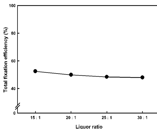
Fig. 8. Effect of liquor ratio on fixation efficiency (%FE).
