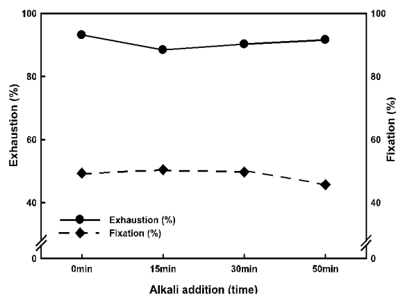
Fig. 9. Effect of process modification on exhaustion (%E) and fixation(%F).
