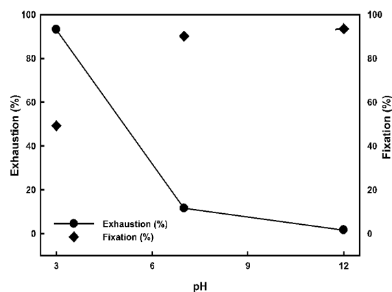
Fig. 3. Effect of pH on exhaustion(%E) and fixation(%F).
