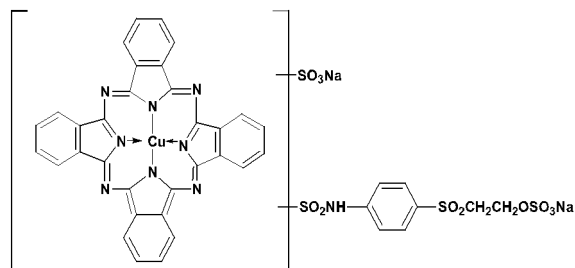
Fig. 1. Structure of the reactive copper phthalocyanine(CuPc) reactive dye.
