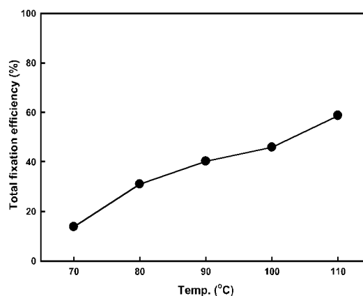
Fig. 6. Effect of temperatures on fixation efficiency (%FE).
