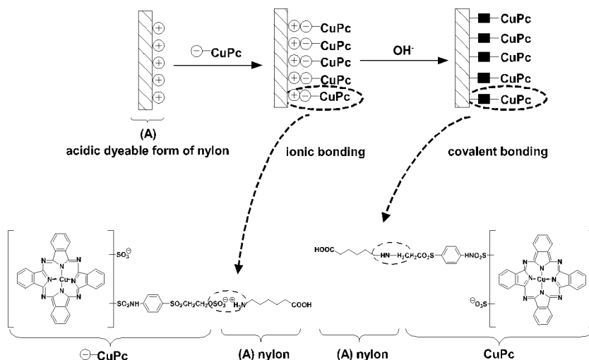
Fig. 2. Reaction mechanism of nylon fiber with copper complex phthalocyanine(CuPc) reactive dye.
