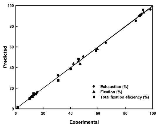
Fig. 13. Experimental and Predicted values of % exhaustion, fixation and total fixation efficiency.
