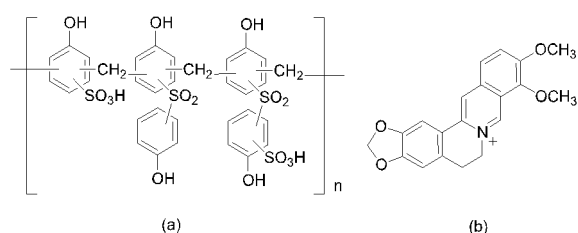
Fig. 1. Structures of (a)syntan and (b)berberine chloride.
