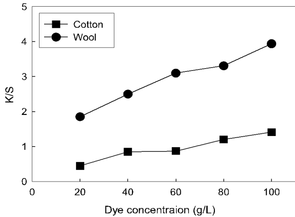
Fig. 4. Effect of dye concentration on K/S values of cotton and wool fabrics dyed with Sasa quelpaertensis extract.(liquor ratio 1:50, dyeing temp. 80°C, dyeing time. 60min, dyeing pH(cotton 11.0, wool 3.0))
