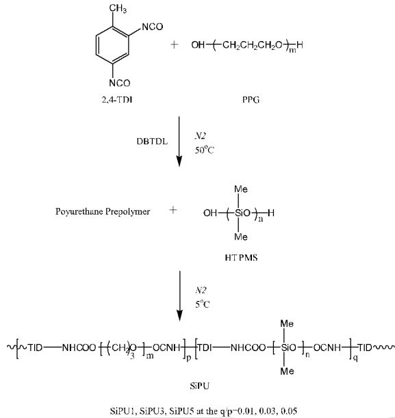
Scheme 1. Formation of synthetic SiPU.
