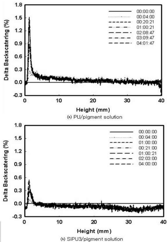
Fig. 3. Delta BS signals of PU/pigment (a) and SiPU3/pigment solutions (b) at leaving time (day:hr:min.).
