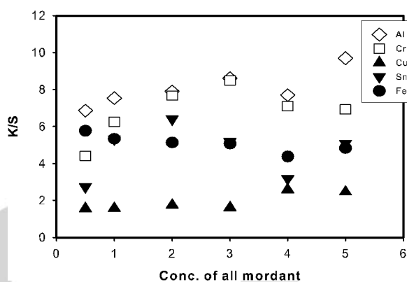
Fig. 7. Relationship between concentration of mordant and K/S values of Wool fabric dyeing with Cochineal under the optimum condition.
