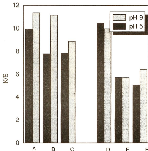
Fig. 7. Relationship between pH's and K/S values of polyester fabrics dyed with C. I. Disperse Yellow 54 under micro wave and 100 °C for 65 min using various carriers, respectively ; A,D : ethylhexyl alcohol, B,E : ethylene glycol, C,F : propylene glycol, A,B,C : micro wave.
