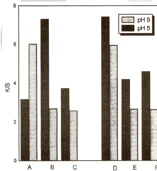
Fig. 5. Relationship between pH's and K/S values of polyester fabrics dyed with C. I. Disperse Red 60 under micro wave and 100℃ for 65 min using various carriers, respectively ; A,D : ethylhexyl alcohol, B,E : ethylene glycol, C,F : propylene glycol, A,B,C : micro wave.
