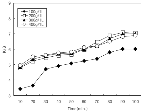
Fig. 4. Relationship between K/S value and material quantity and dyeing time.
