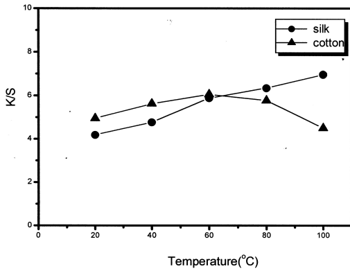
Fig. 3. K/S Value of fabrics dyed by Rhus vernicia extract at various dyeing temp(30min).
