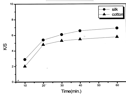
Fig. 4. K/S Value of fabrics dyed by Rhus vernicia extract at various dyeing time(60 °C).
