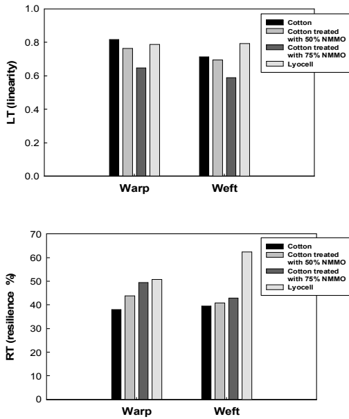
Fig. 4. Tensile property(linearity LT and resilience RT) of various cellulosic fibers.
