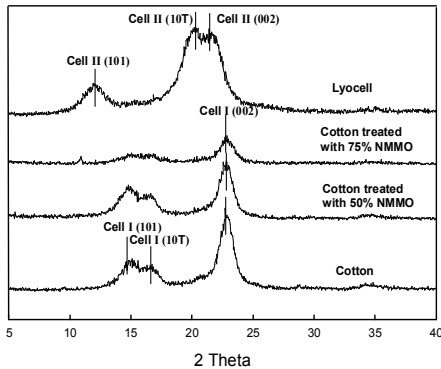
Fig. 1. X-ray diffraction patterns of various cellulosic fibers.
