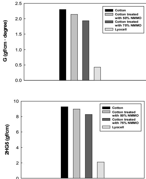
Fig. 6. Shearing property (shearing rigidity G and hysteresis width at \Phi=5 degree) of various cellulosic fibers.
