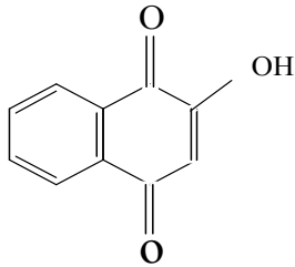
Fig. 1. Structure of Lawsone.
