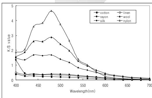
Fig. 2. Changes of K/S values of the fabrics dyed with balsamine extracts at 40 °C for 10 minutes
