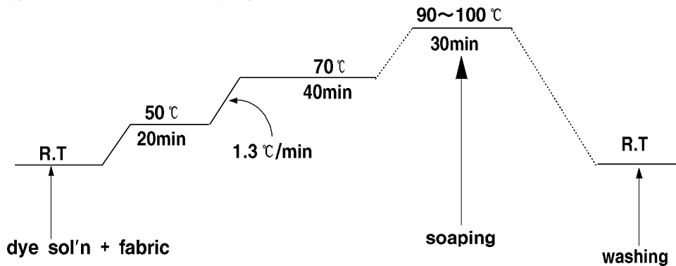
Scheme 4. Dyeing diagram of reactive dye.
