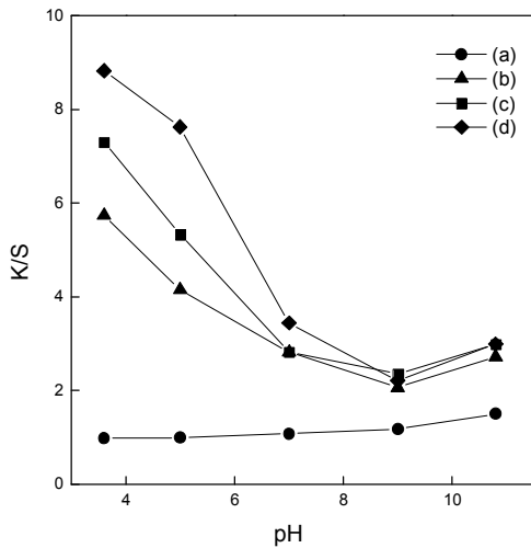
Fig. 6. Effect of pH on the K/S values of the fabrics treated with glutaraldehyde/softener at various chitosan concentrations ; (a) control, (b) 0.5%, (c) 0.7%, (d) 1.0%. (dyeing conditions : 2% owf C. I. Reactive Red 120, Na 2 SO 4 10g/ℓ, 70°C)
