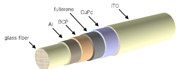
Fig. 3. Schematic illustration of the solar cell fiber.
