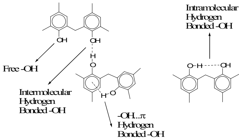
Scheme 3. Possible hydrogen bonded species in phenolic dimer.
