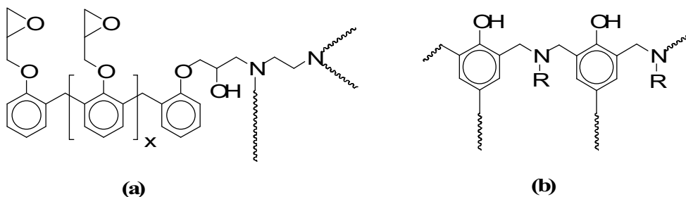
Scheme 1. Structures for typical phenolic resins.
