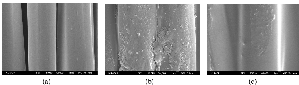
Fig. 4. SEM images of (a) untreated and grafted PET fabric with (b) VP (11.6%G) and (c)ACMO (25.3%G).
