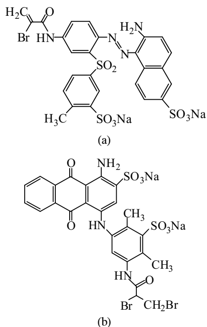
Scheme 2. Molecular structures of (a) C.I. Reactive Red 84 and (b) C.I. Reactive Blue 50.
