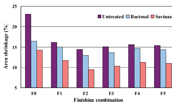
Fig. 4. Shrinkage of finished and unfinished wool/cotton blend fabrics.
