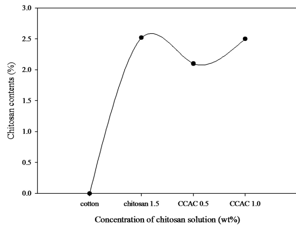
Fig. 8. Chitosan contents of 1.5 wt% chitosan fiber and CCAC(calcium alginate: 0.5 wt%, 1.0 wt%) fiber.
