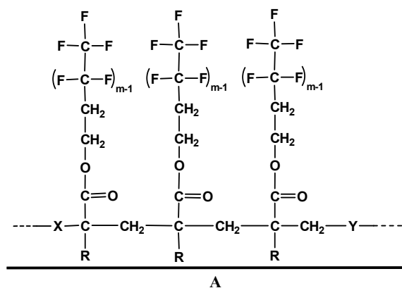
Figure 1. Fluorocarbon repellent agent on fiber surface. M = 8-10, X and Y are comonomers, mainly stearylacrylates. R = H and CH 3 (polyacrylic or polymethacrylic acid esters). A is the fiber surface.
