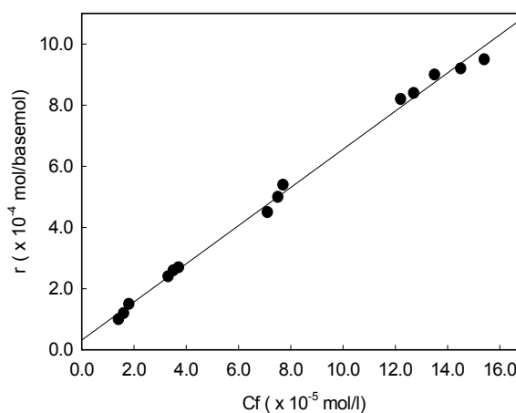
Figure 5. Isotherms for binding of Red 18 with PVP in an acetate buffer solution(pH 4.2) at 30°C.
