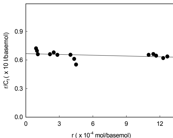
Figure 6. Scatchard plots for binding Red 18 with PVP in an acetate buffer solution. (pH 4.2, I=0.02) at 30°C.
