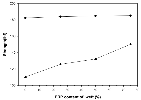
Figure 3. Effect of FRP content of weft on tensile strength (● : direction of warp, ▲ : direction of weft).
