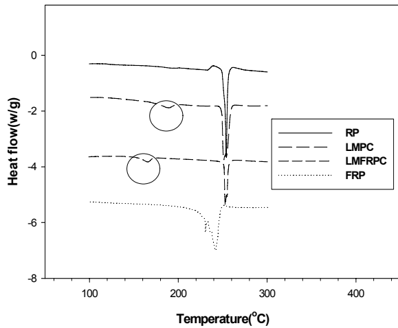
Figure 1. DSC thermograms (in N 2 ) of RP, LMPC, LMFRPC and FRP.
