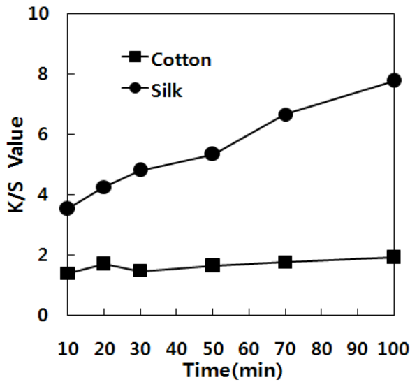
Figure 4. Effect of dyeing time of cotton and silk fabrics dyed with methanol extracts from Juniperus chinensis heartwood on the K/S values (0.5%(o.w.b), 60°C).
