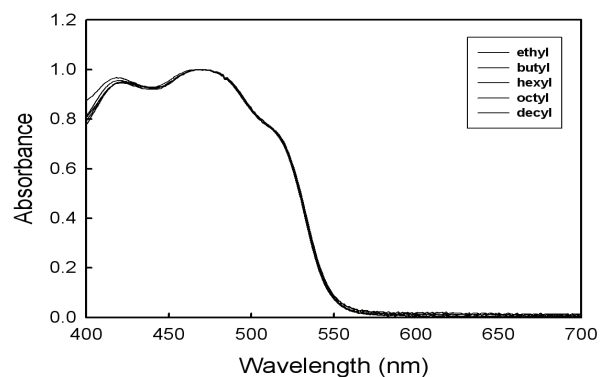
Figure 4. UV-Visible spectra of super hydrophobic orange dyes.
