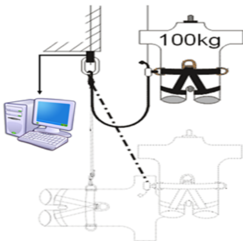
Figure 3. Test stand used for dynamic load test of the absorber.
