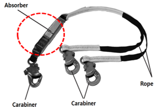
Figure 1. Form of energy absorbing lanyard.
