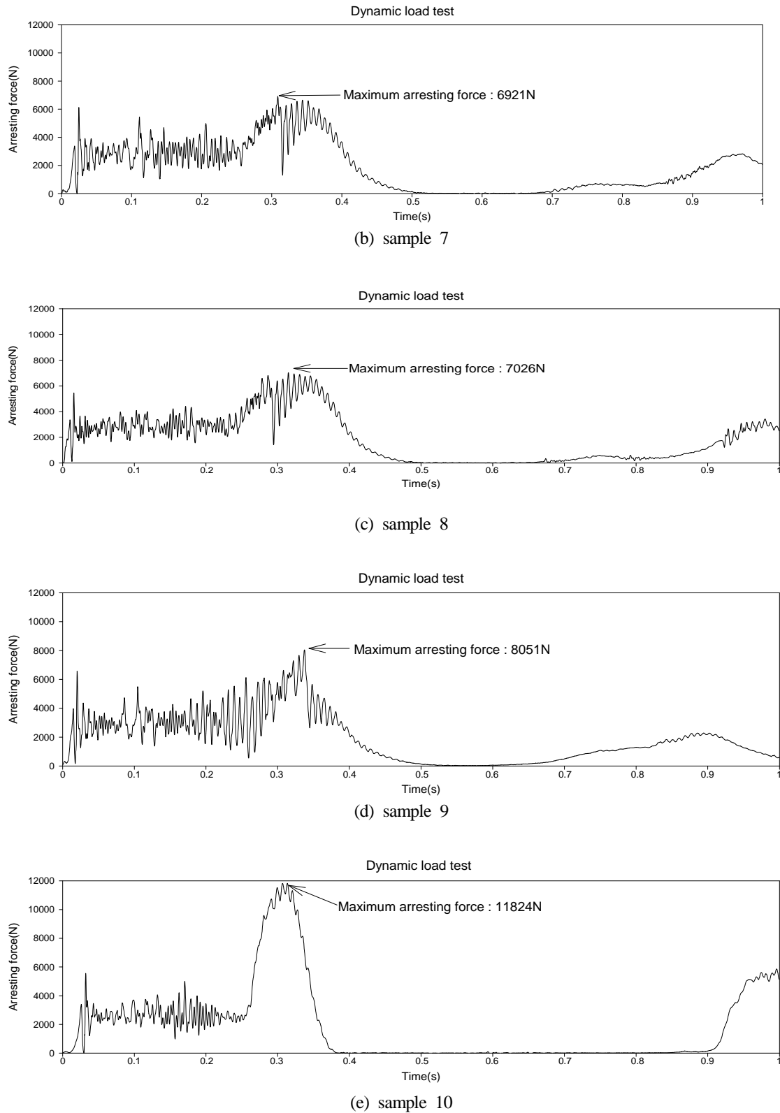
Figure 6. The dynamic load test of absorber (a) sample 6 interlace filament density 55, (b) sample 7 interlace filament density 54, (c) sample 8 interlace filament density 53, (d) sample 9 interlace filament density 52, (e) sample 10 interlace filament density 51.
