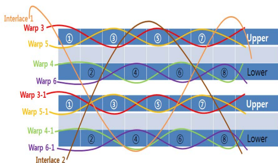
Figure 2. Structure of narrow width fabrics.
