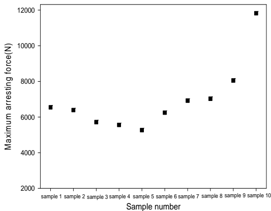
Figure 7. Influence for conditioning on the maximum arresting force(N) value of the dynamic load of absorber type interlace filament density.
