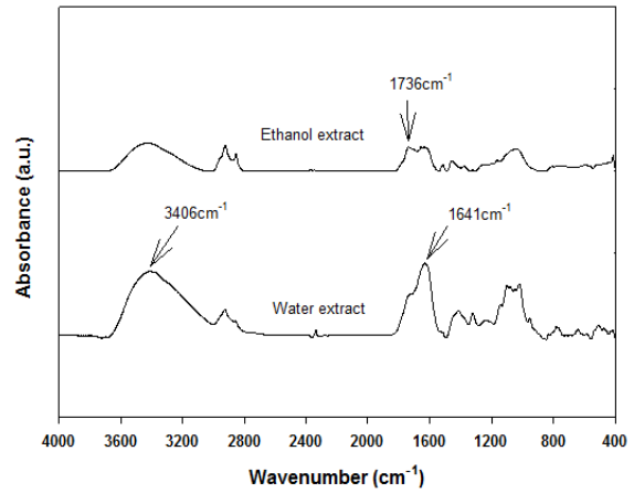
Figure 3. FT-IR spectra of Houttuynia cordata extracts.
