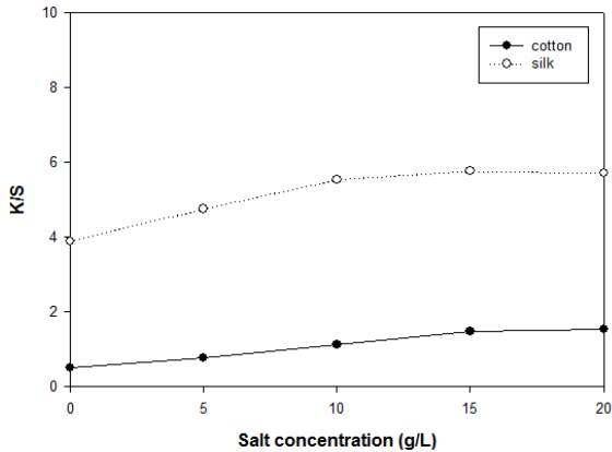
Figure 4. Effect of salt concentration on K/S values of dyed fabrics.
