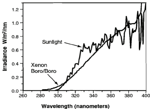
Figure 2. Spectrum of xenon arc lamp with boro/boro filter and sunlight 8) .
